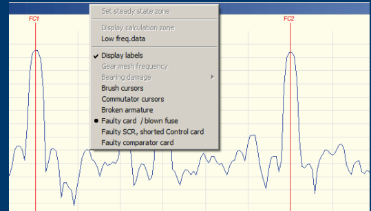
ATPOL II™ automatically identifies and reports common DC motor faults, such as broken armature, faulty SCR's, etc.
